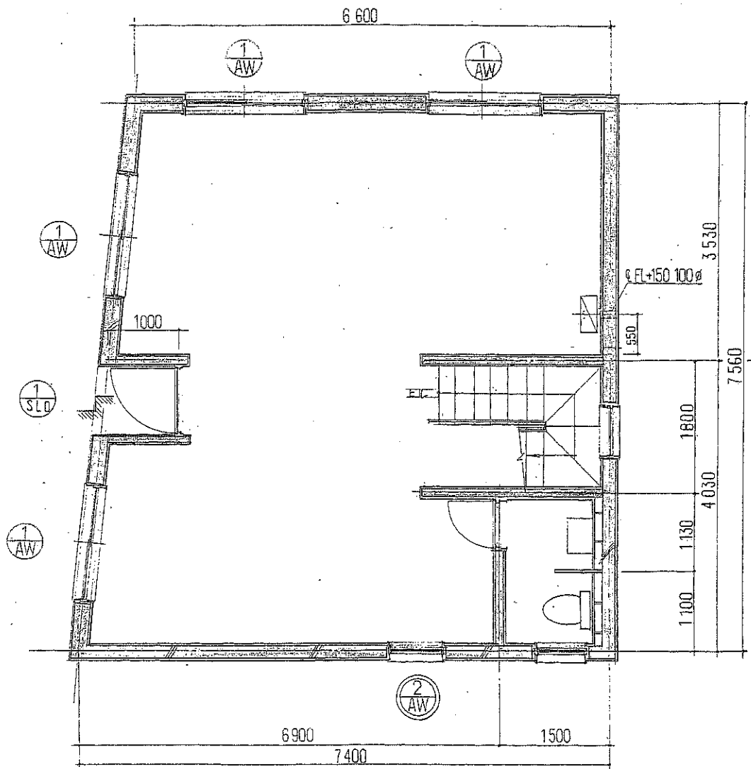
1F PLAN S=1/50
