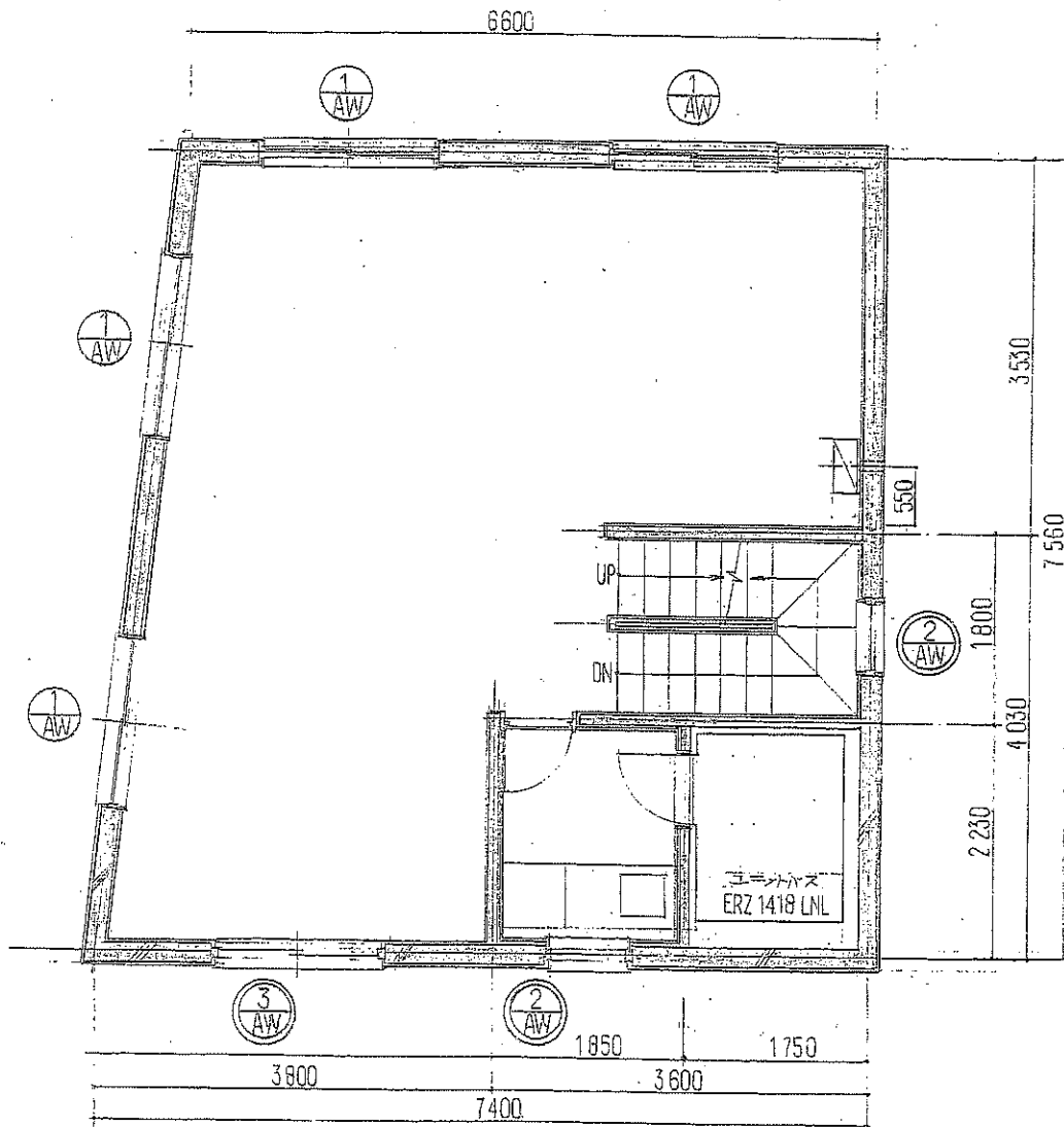
2F PLAN S = 1/50
